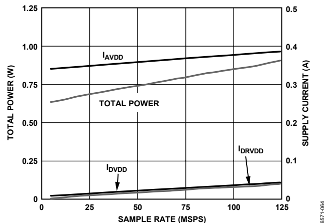
Figure 64. AD9627-125 Power and Current vs. Sample Rate
