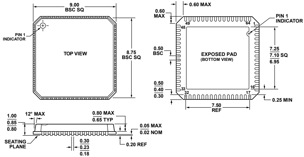
COMPLIANT TO JEDEC STANDARDS MO-220-VMMD-4 Figure 93. 64-Lead Lead Frame Chip Scale Package [LFCSP_VQ] 9 mm × 9 mm Body, Very Thin Quad (CP-64-3) Dimensions shown in millimeters
