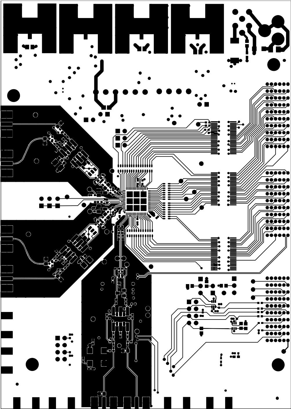
Figure 85. Evaluation Board Layout, Primary Side
