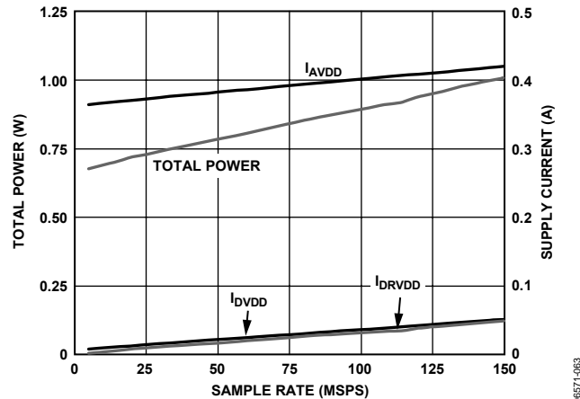
Figure 63. AD9627-150 Power and Current vs. Sample Rate
